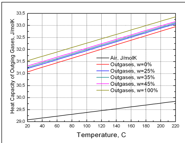
Fig. 6. Dependences of heat capacities of air and exhaust gases (at \alpha = 1 ) by temperature and firewood's moisture.
